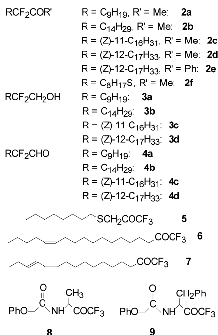
Scheme 1. Structures of compounds 2–9 synthesized as potential inhibitors of esterases.
